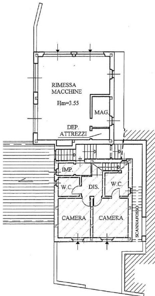
PIANO TERRA
