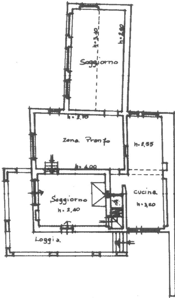
PIANO TERRENO
