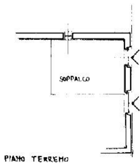
PIANO TERRENO
