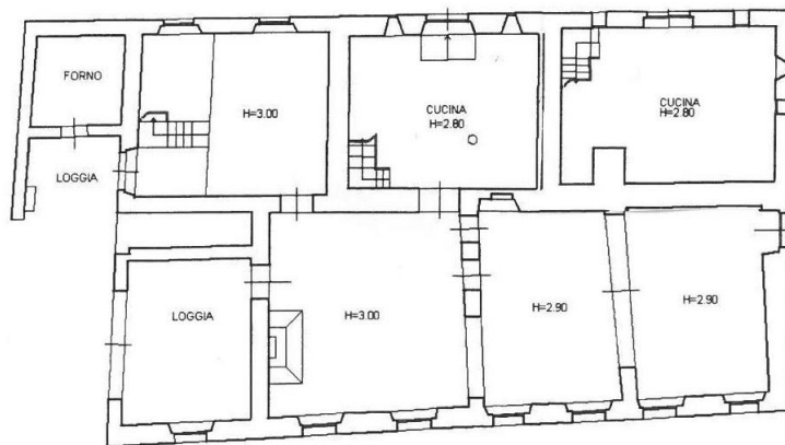
PIANO TERRA
