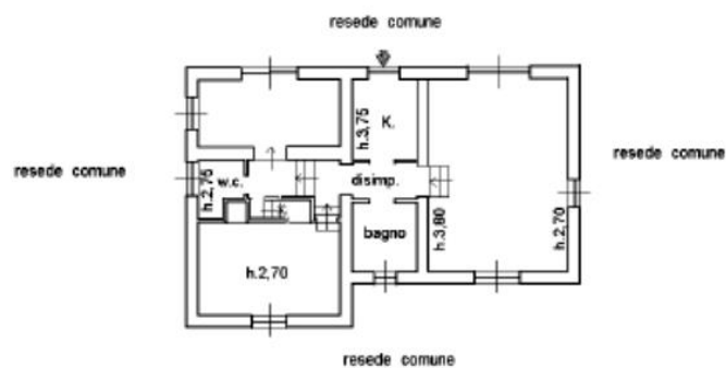
PIANO TERRA (T)
